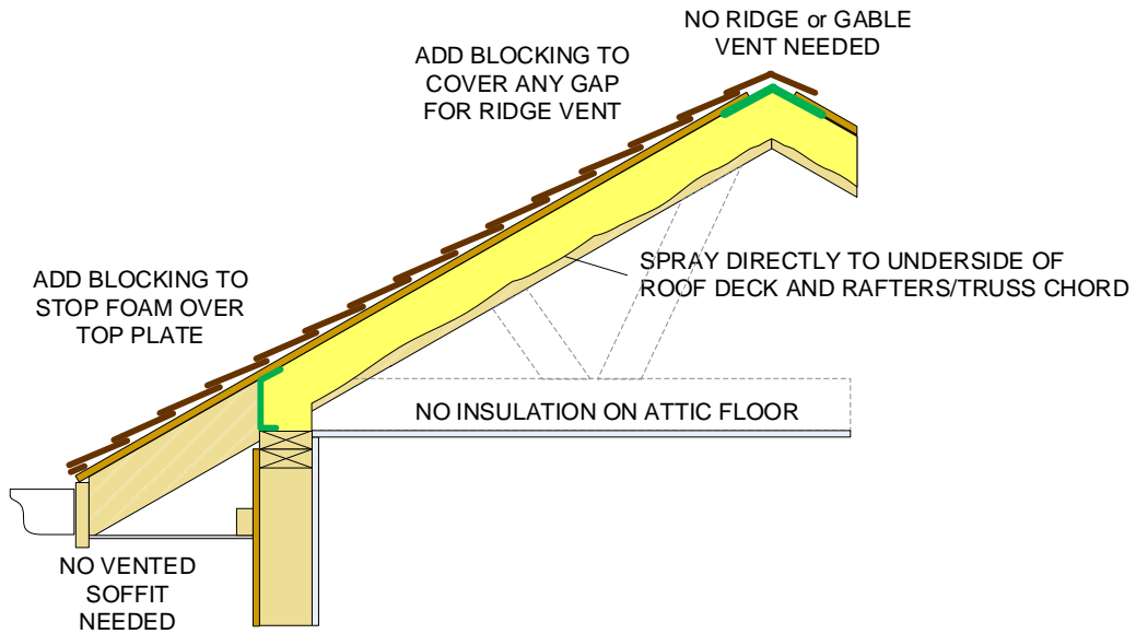
Figure 1 - Typical installation diagram for SPF applied to underside of roof deck to create an unvented attic
