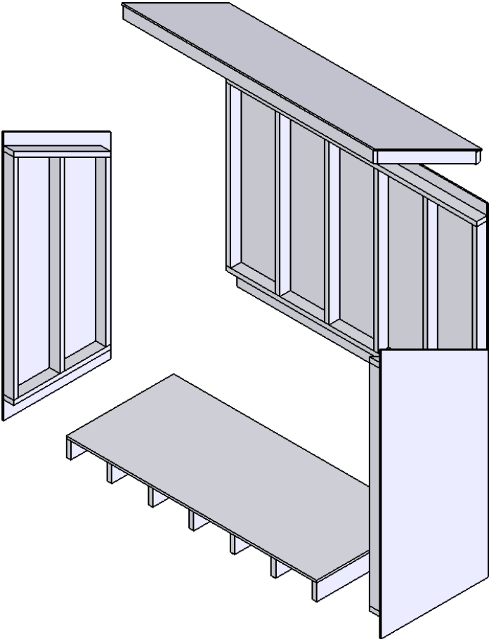
EXPLODED VIEW
